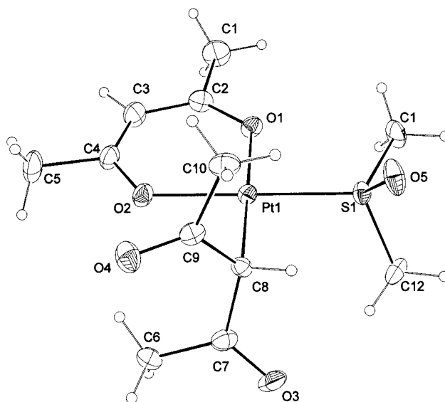
Figure 4. Molecular structure of one out of three independent molecules (molecule 2 ) in the asymmetric unit of compound 2
