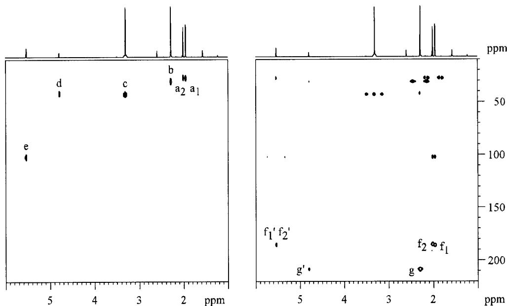
Figure 1. ^1H - ^{13}C HETCOR (left) and ^1H - ^{13}C long range HETCOR (right) spectra of 2 . Hydrogen bearing carbon atoms of O,O' -chelated acac ( a_1 , a_2 , and e ), C\gamma -bonded acac ( b and d ) and DMSO ( c ) were detected by ^1H - ^{13}C HETCOR while the carbonyls of the O,O' -chelated acac and the C\gamma -bonded acac could be assigned according to cross peaks with methyls ( f_1 , f_2 , and g , respectively) or according to cross peaks with C\gamma -H ( f_1' , f_2' , and g' , respectively) in the ^1H - ^{13}C long range HETCOR spectrum
