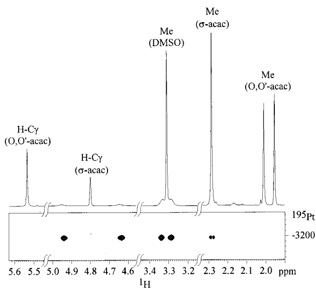
Figure 3. ^1\text{H}\text{-}^{195}\text{Pt} -HETCOR spectrum of 2 acquired without ^{195}\text{Pt} decoupling during acquisition. For clarity, ^1\text{H} projections are not on the same vertical scale
