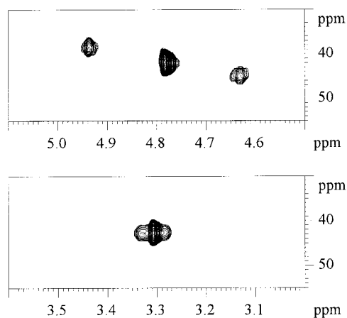
Figure 2. Expansions of ^1\text{H}\text{-}^{13}\text{C} HETCOR spectrum of 2 showing ^{195}\text{Pt} satellites relative to the \text{C}\gamma -bonded acac (above) and the DMSO methyl groups (below)
