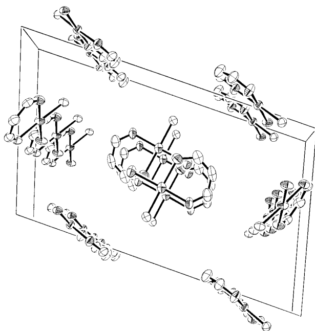
Figure 5. Unit cell projection along the a -axis showing alternating 2b molecules staggered by ca. 180^\circ and stacked inside the channel resulting from the propagation of molecules of 2 (top and bottom) and 2a (sides). Only ligand atoms in the coordination plane are shown (see Supporting Information, S4 for the same projection with all atoms except hydrogen)
